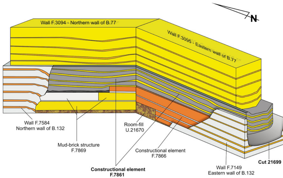
Figure 31.53. Schema of the northeastern corner of Sp.602, with the different retention wall constructions before the construction of B.77 (illustration by Arek Klimowicz).
